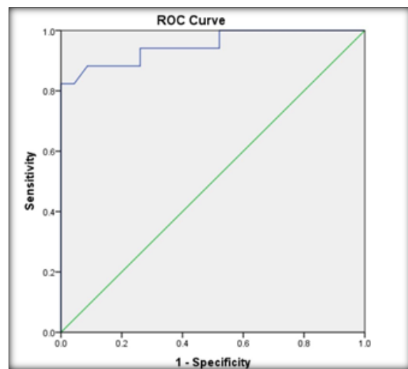
Figure 1: ROC curve for urine NGAL
